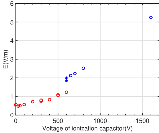
Figure 3. Operational space for pure Ohmic heating start-up and ECH assisted start-up on J-TEXT. A circle means the discharges were successful while an asterisk indicates the shot failed. The blue represents that it is a pure Ohmic heating start-up while the red represents EC assisted start-up
