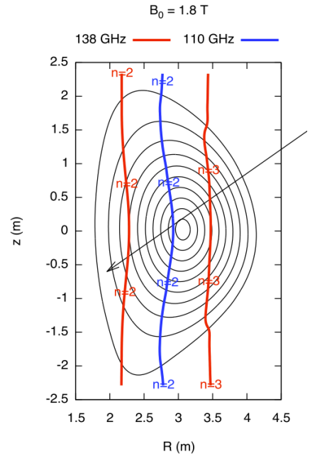
Fig. 6. EC resonances for B_0=1.8T (cases 4, 5)
