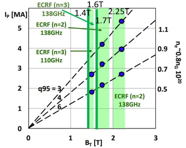
Fig. 1. Possible operational path for the rise to 5.5MA in the Initial Research phase. Adapted from [1]
