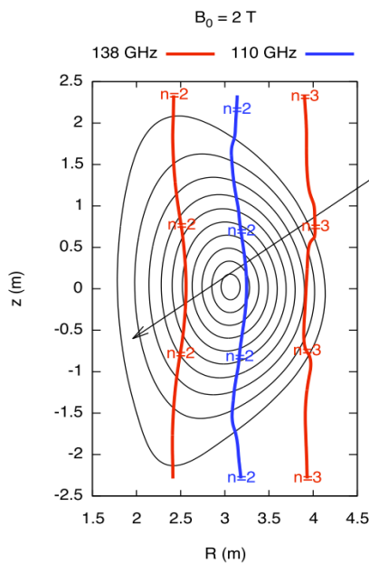
Fig. 5. EC resonances for B_0=2T (cases 2, 3).
