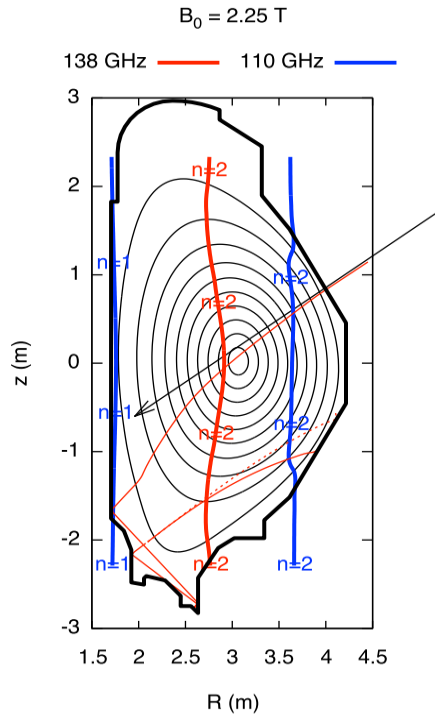
Fig. 4. Beam trajectory (red lines) and EC resonances for the harmonic n for scenario 2 at nominal magnetic field. The black arrow represents the initial injection direction. Applies to case 1.
