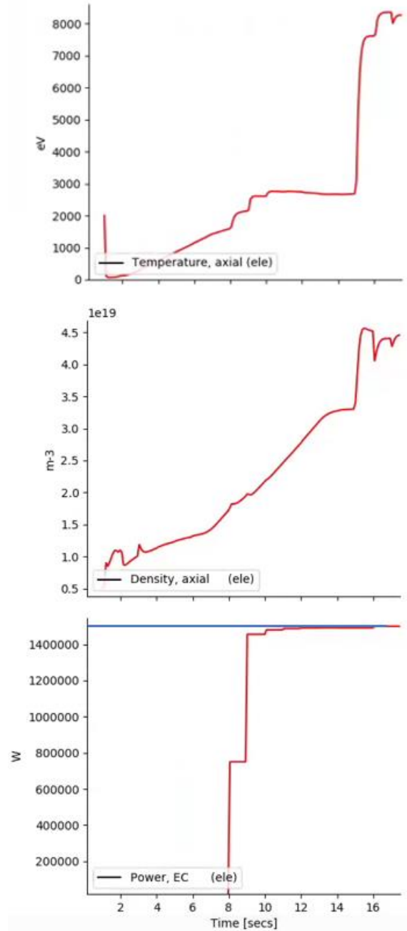
Fig. 3. Time evolution of the axial electron temperature (top), of the axial density (mid) and of the absorbed EC power (bottom) for case 6 simulation in Table 1.
