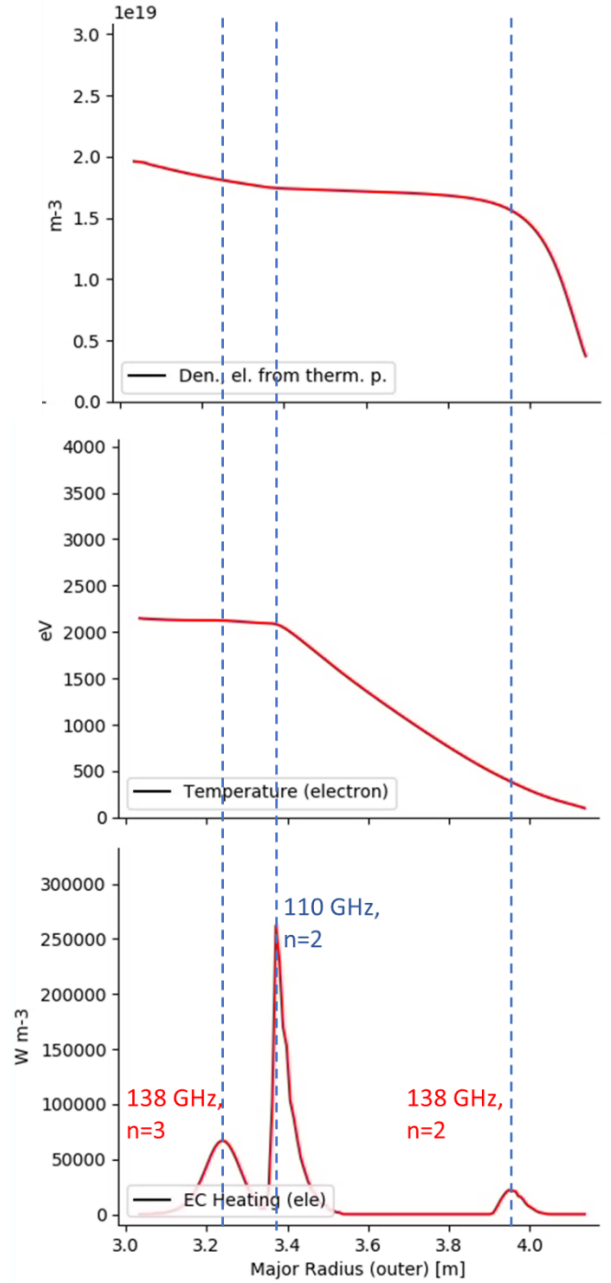
Fig. 9. Density, temperature and absorption profiles for case 6b
