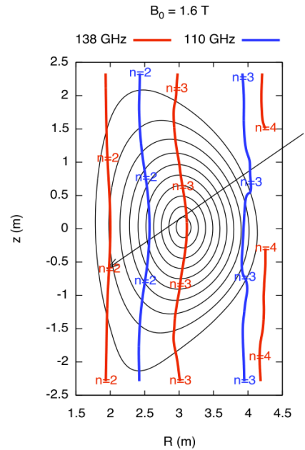
Fig. 7. EC resonances for B_0=1.6 T (case 8).
