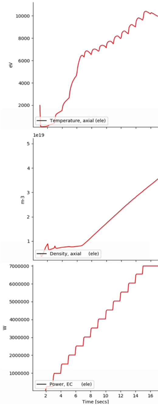
Fig. 2. Time evolution of the axial electron temperature (top), of the axial density (mid) and of the absorbed EC power (bottom) for case 1 simulation in Table 1.
