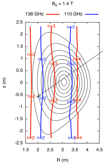
Fig. 8. EC resonances for B_0=1.4T (case 9)
