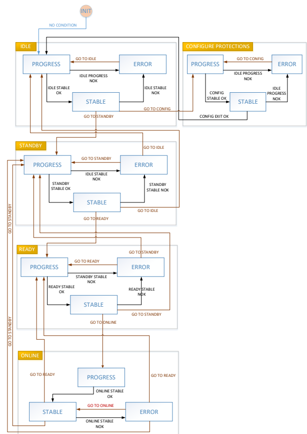
Fig. 2. ECPC State Machine.
