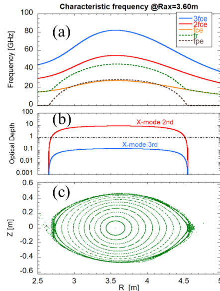
Fig. 1. (a) Radial profile of characteristic frequencies in the major radial direction in the LHD horizontal cross-section at B_t = 1 T and R_{ax} = 3.60 m. The blue line is the 3rd harmonic 3f_{ce} , the red line is the 2nd harmonic 2f_{ce} , the yellow line is the fundamental f_{ce} , the green dotted line is the right-hand X-mode cutoff frequency, and the brown dotted line is the electron plasma frequency f_{pe} . Here the electron density is calculated as n_{e0} = 1 \times 10^{19} \text{ m}^{-3} at the center. (b) Optical thickness at T_e = 2 keV, where the X-mode 2nd harmonic f_{ce} exceeds 1 almost everywhere in the plasma confinement region. (c) Closed flux surface per \rho = 0.1 and ergodic region in vacuum.
