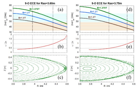
Fig. 11. (left) Radial distribution at R_{ax}=3.60 m and (right) R_{ax}=3.75 m. (a, d) Second harmonic cyclotron frequencies at B_t = 1 T, 1.2 T and 1.375 T. The orange and the light blue horizontal lines indicate the Q- and V-band measured channels' frequencies, respectively. (b, e) Iota distribution (c, f) Magnetic closed flux surfaces for every \rho=0.1 .
