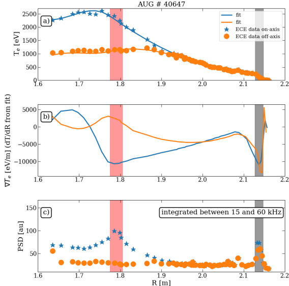
Figure 7. AUG #40647: a) Profile from the electron temperature T_e measured with ECE in symbols and the corresponding fits in solid lines. b) Gradients of the electron temperature fits. c) Amplitude distribution of Fourier filtered data between 15 and 60 kHz. The two shaded regions correspond to the maximum perturbation amplitude in the core (in red) and at the edge (in black).
