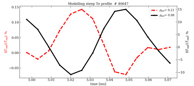
Figure 8. ECRad modeling: radiation transport for input gradients similar to #40647 in the phase with largest central T_e gradient, corresponding to the phase with maximum central heating
