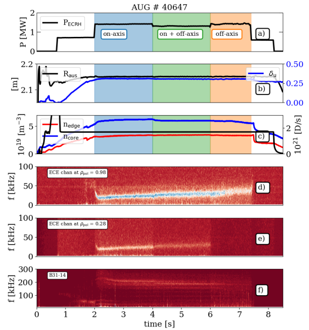
Figure 6. AUG #40647: Temporal evolution of plasma parameters during EDA H-mode. a) ECRH heating scheme. b) Outer plasma boundary and upper triangularity. c) edge and core densities together with the deuterium fuelling. d) Spectrogram of the edge ECE channel. e) Spectrogram of the ECE core channel. f) Spectrogram of the magnetic coil B31-14 measuring changes in the radial magnetic field. Time intervals of different heating schemes are marked in colored surfaces: blue - on-axis heating; green - on and off-axis heating; orange - off-axis heating.
