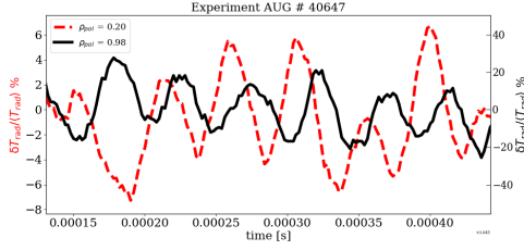
Figure 9. AUG #40647: Phase and amplitude for core and edge radiation temperature fluctuations \delta T_e / \langle T_e \rangle obtained from the raw ECE data in the core \rho_{pol} = 0.2 (red) and at the edge at \rho_{pol} = 0.98 (black).
