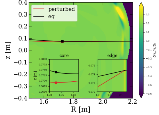
Figure 11. 2D density contour plot with density perturbation at the edge used in the forward model. The ECE ray is refracted at the edge which can be seen in the zoomed picture and the resonance (in red) is displaced with respect to the equilibrium (black) position.
