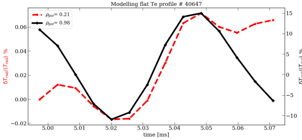
Figure 10. Modeled radiation transport for the discharge # 40647 in the phase of off-axis heating where the Te profile is flat compared to the case with on-axis heating.
