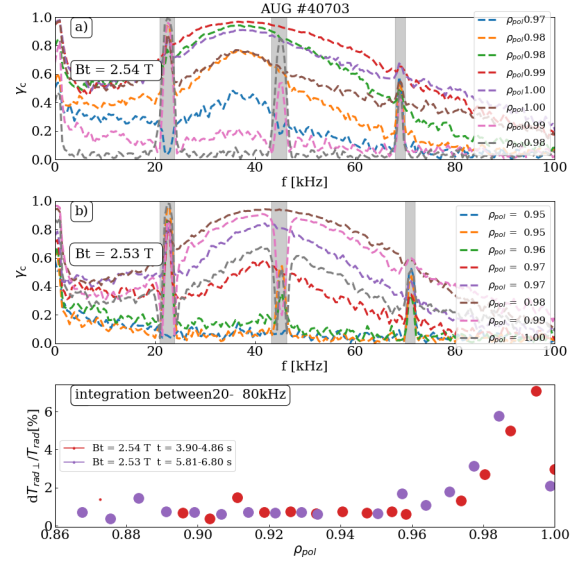
Figure 2. AUG #40703 a) Cross-coherence between subsequent CECE channels for magnetic field strength of 2.54 T. b) Cross-coherence between subsequent correlation ECE channels for magnetic field strength of 2.53 T. c) Relative radiation temperature fluctuations integrated between 20 and 80 kHz from the CECE measurements for B_t = 2.54 T in red and for B_t = 2.53 T in magenta, respectively. Grey regions are marking peaks of strong noise in the channels.
