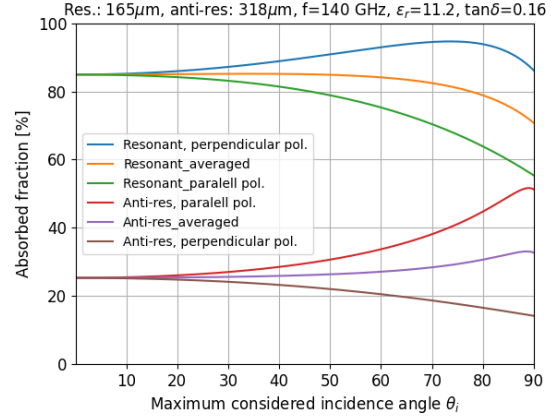
Figure 8. Modelled isotropic stray radiation response with input data from Fig. 7. Upper traces: resonant, 165\ \mu\text{m} , lower traces: anti-resonant, 318\ \mu\text{m} . The absorbed fractions are plotted as a function of considered range of incident angles, e.g. \theta_i = 0^\circ is normal incidence while \theta_i = 20^\circ includes all incidence angles up to 20^\circ . For each thickness the response to perpendicular and parallel polarisation is plotted. The averages of these (label 'averaged') is the overall isotropic stray radiation response.
