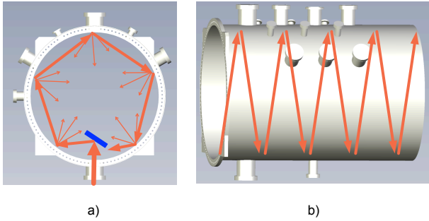
Figure 1. Conversion of collimated beam to stray radiation.
