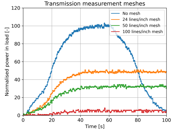
Figure 6. Insertion loss of wire meshes using the caloric load. MISTRAL not at vacuum: to avoid possible arcing the calibration pulse (blue) was limited to one minute.
