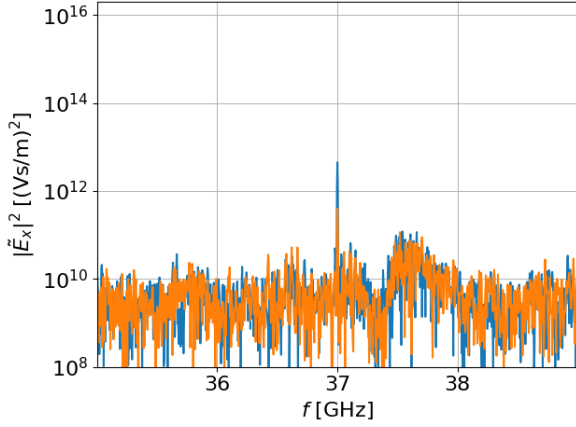
(a) Two spectra in the linear pump intensity regime. The orange line is for I_0 = 10^3 \text{ W/m}^2 and the blue line is for I_0 = 10^4 \text{ W/m}^2 . Ions are mobile in both.
