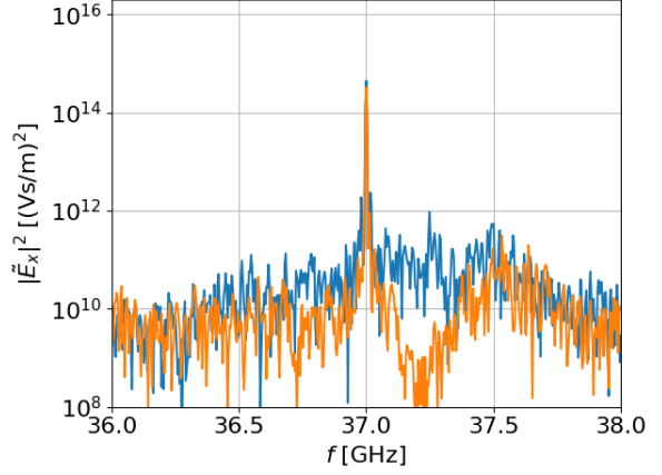
(b) The pump wave intensity is I_0 = 10^5 \text{ W/m}^2 , the orange line is for immobile ions and the blue line is for mobile ions. Notice the difference near 37.25 GHz and near the pump, see the zoom in figure 2c.
