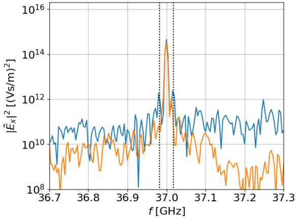
(c) Same as figure 2b but zoomed in near the pump frequency. Notice the symmetric peaks shifted by \sim 20 \text{ MHz} , marked by vertical dotted lines and visible only when ions are mobile.
