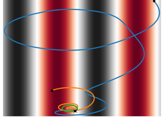
(b) Examples of electron trajectories at different EBW electric field amplitudes, an instance of the wave field is shown in the red-black heat map. The lines are for |A| \ll 1 (green), |A| \approx 1 (orange) and |A| \gg 1 (blue). The cross marks the starting position and circles are ending positions after 2 cyclotron periods. Trajectories are calculated using a Boris update scheme.
