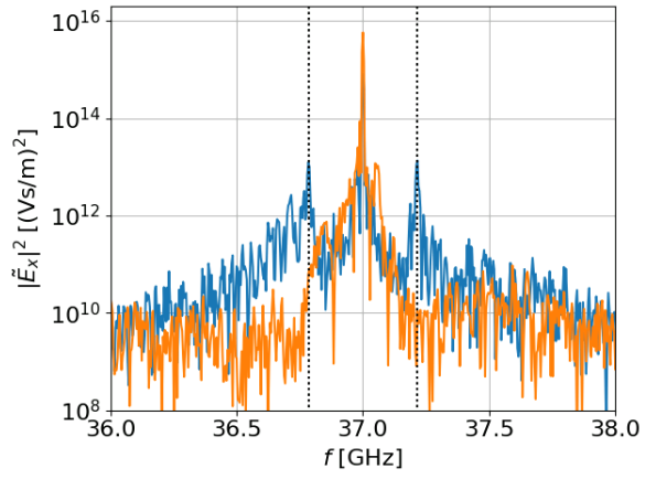
(d) The pump wave intensity is I_0 = 10^7 \text{ W/m}^2 . The orange line is for immobile ions and the blue line is for mobile ions. Notice the development \sim 0.2 \text{ GHz} from the pump when the ions are mobile.
