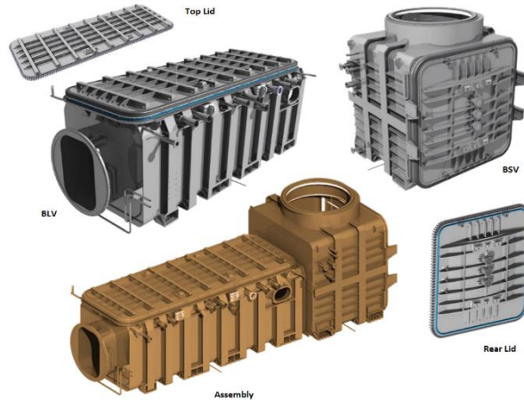
Main welded assemblies of the Neutral Beam Vacuum Vessel. procured
